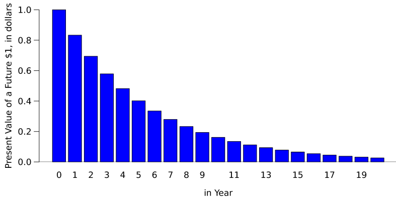
Figure 1: Discounting $1
